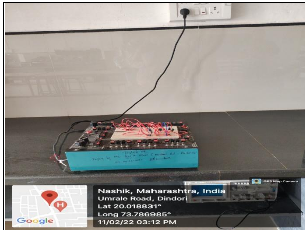
Breadboard Circuit
